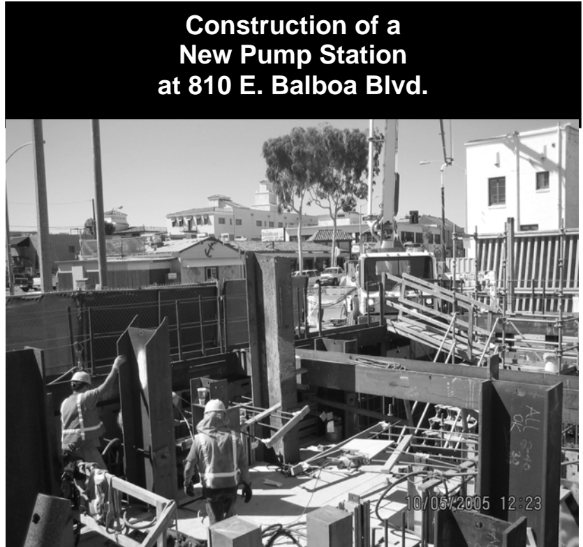
Installation of structural walls.
